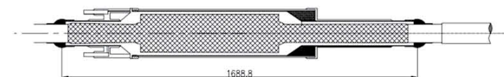
110kV insulation intermediate joint
