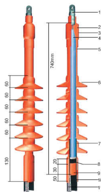
26/35kV single-core outdoor termination in stallion drawing
