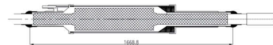
110kV straight through intermediate joint
