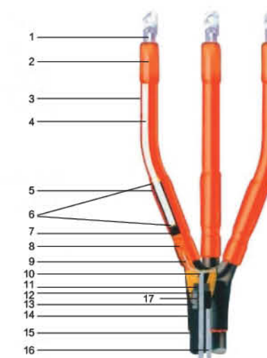
8.7/15kV three-core termination structure diagram
